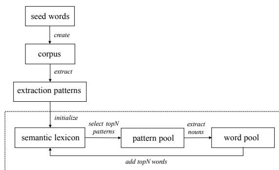
Figure 1: Schematic overview of bootstrapping process.
