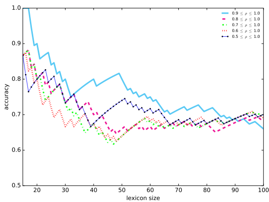
Figure 7: Graph that shows the accuracy when learning 100 words for the top 10% to top 50% verbs when scoring candidate words with BASILISK’s AvgLog ( S_b ).
