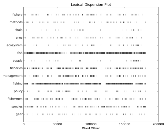
Figure 2: The lexical dispersion plot shows how often a word, displayed on the y-axis, occurs in the cleaned corpus. The x-axis displays the position within the corpus from beginning to end.
