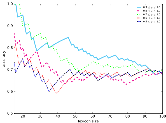
Figure 8: Graph that shows the accuracy when learning 100 words for the top 10% to top 50% verbs when scoring candidate words with Pointwise Mutual Information ( S_{pmi} ).
