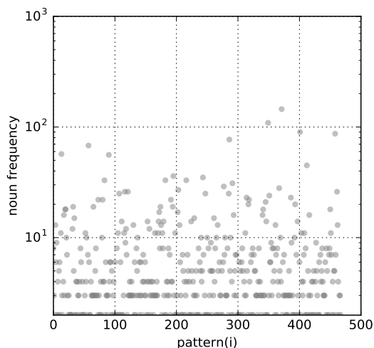
Figure 6: The frequency of nouns in an extraction pattern. The x-axis shows the number of extraction patterns found in our corpus (468). The y-axis shows the number of nouns grouped within that pattern.
