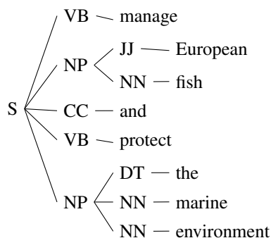
Figure 3: Parse tree for the noun phrase European fish with its accompanying transitive verb manage and noun phrase the marine environment with transitive verb protect . Both NPs occur as a direct object.
